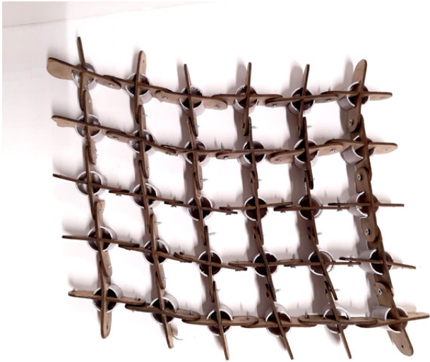
FIGURE 16: Flat Assembled Hinged-Joint Shell
