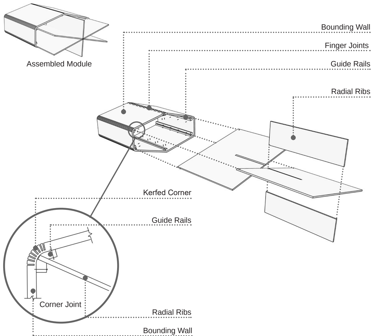
FIGURE 32: Module Details
