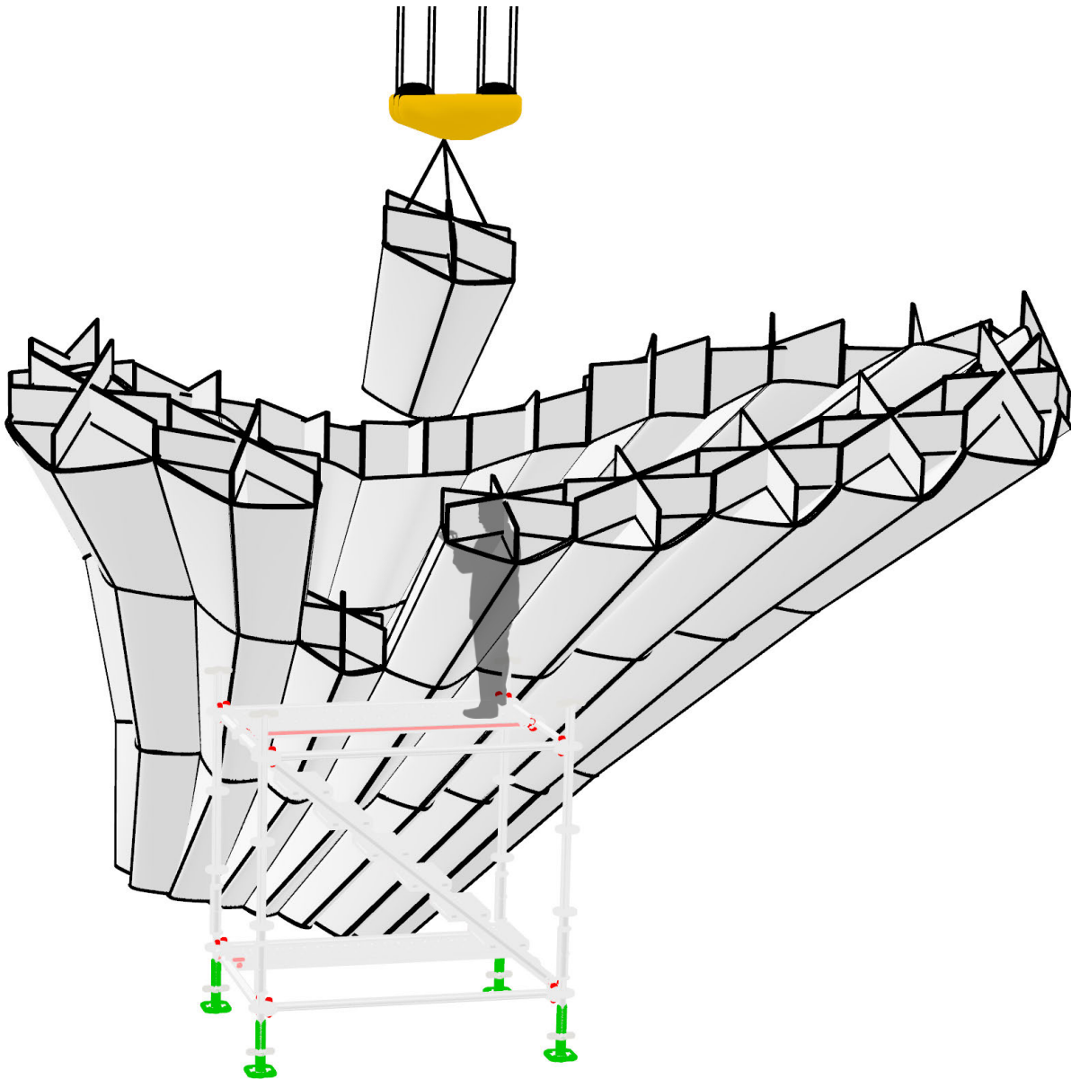
FIGURE 33: Construction Procedure
